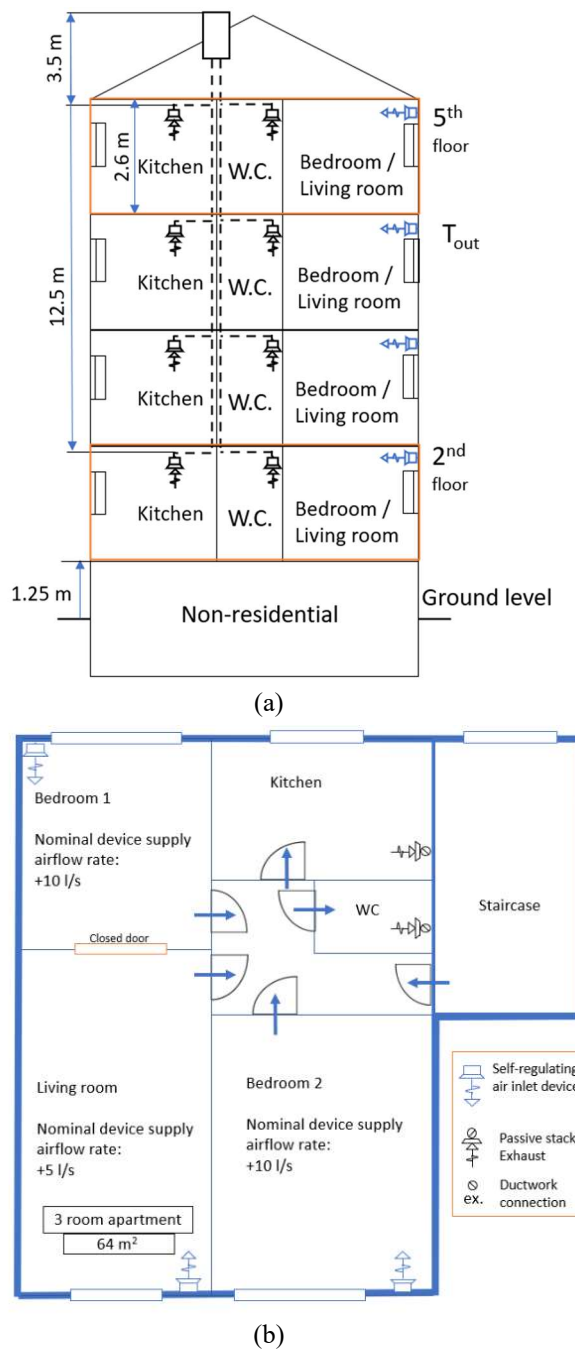
Figure 1: The building ventilation system design (a); The building apartment level ventilation system design (b). (Kravchenko et al. 2022)
