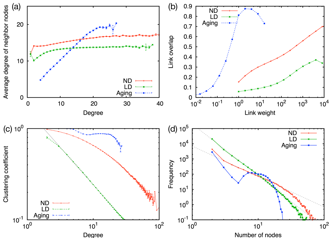
Fig 5. Relations of various network characteristics. (a) Average degree of neighboring nodes as a function of degree, (b) link overlap as a function of link weight, (c) local clustering coefficient as a function of degree, and (d) community size distribution for the ND, LD, and aging models. In (c) a fitting line corresponding to x^{-0.82} is also shown. In (d) communities are identified using the link community detection method. Fitting by power laws with exponent -3.4 and -2 are shown as guides to the eyes.
