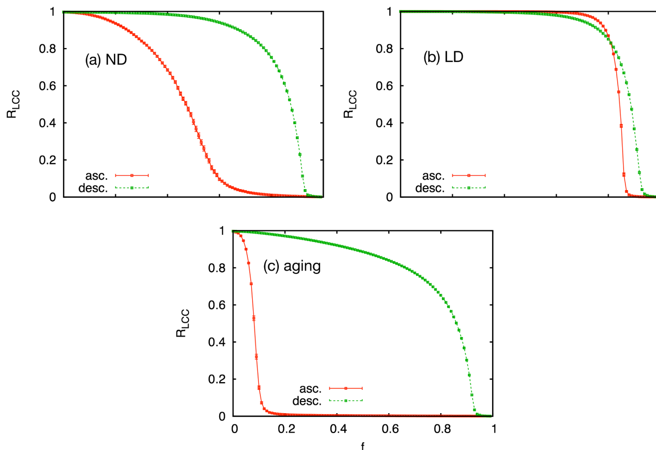
Fig 3. Link percolation analysis. Link percolation analysis for the (a) ND, (b) LD, and (c) aging models. We plot the relative size of the largest connected component, R_{LCC} , as a function of the fraction of removed links f . Red solid (green dashed) curve corresponds to the case when links are removed in ascending (descending) order of link weights. The error bars show standard errors.
