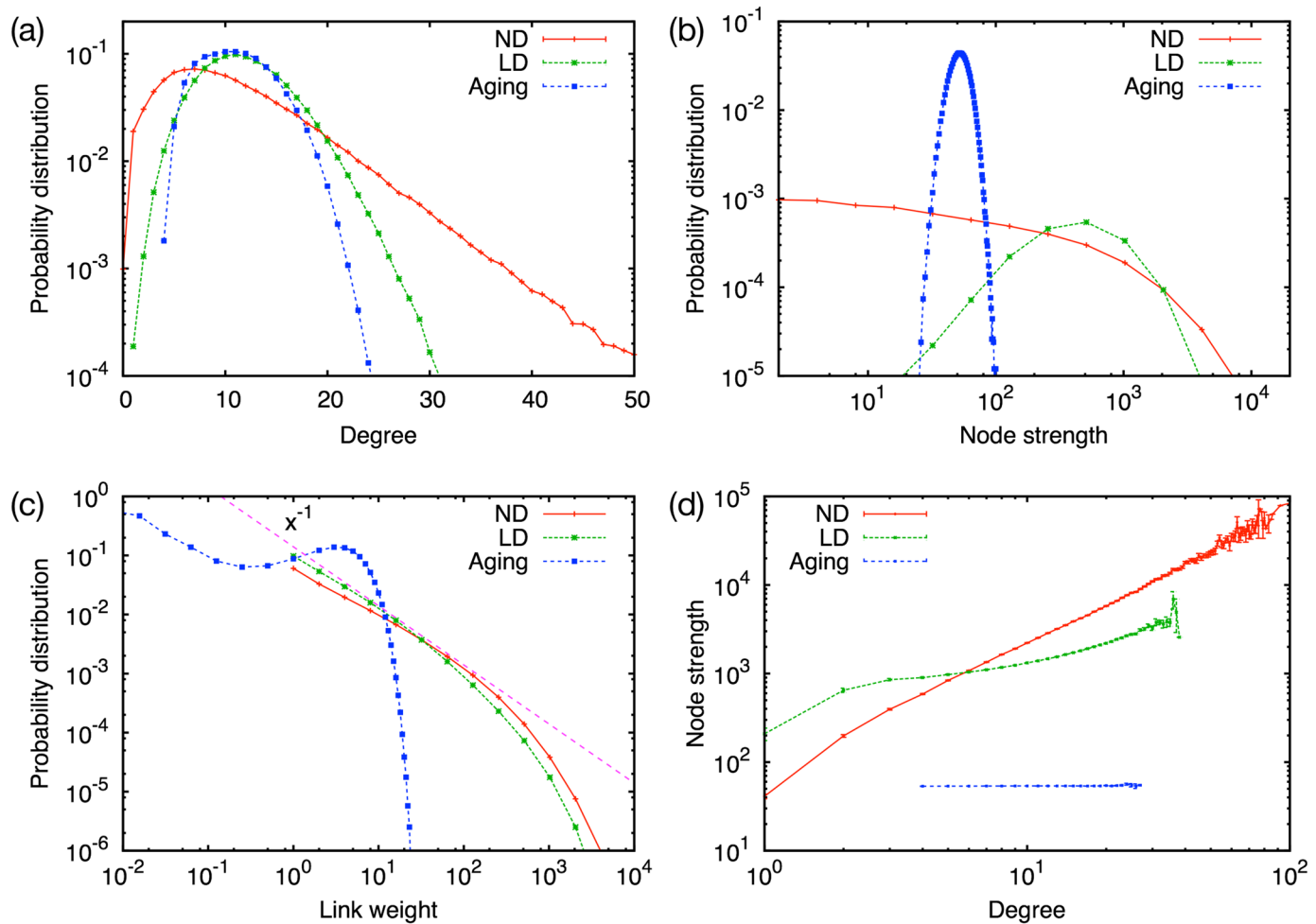
Fig 4. Local network properties. (a) Degree distributions, (b) node strength distributions, (c) link weight distributions, and (d) correlations between node strength and degree for the ND, LD, and aging models. In (c), a fitting line of x^{-1} is also shown.
