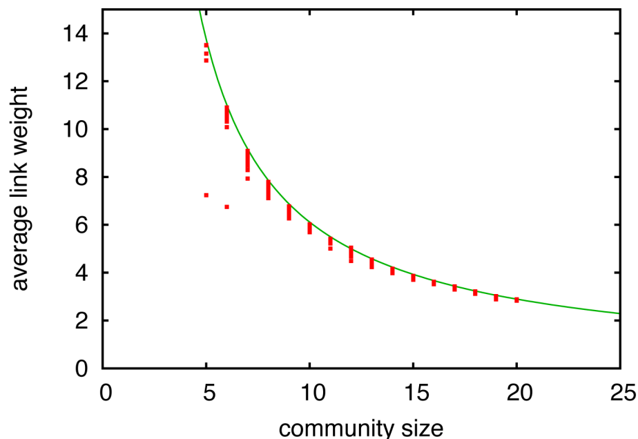
Fig 2. Average link weight of intra-community link as a function of the community size. Communities are obtained from a single run for the aging model and each point corresponds to a community. A fitting function proportional to 1/(n-1) is also shown. For this plot, we used an intermediate solution obtained by the Louvain method because the final solution does not show a clear convergence of the data points to a single curve but to a few curves. It is probably because multiple communities are merged in the final solution due to the resolution limit [16].
