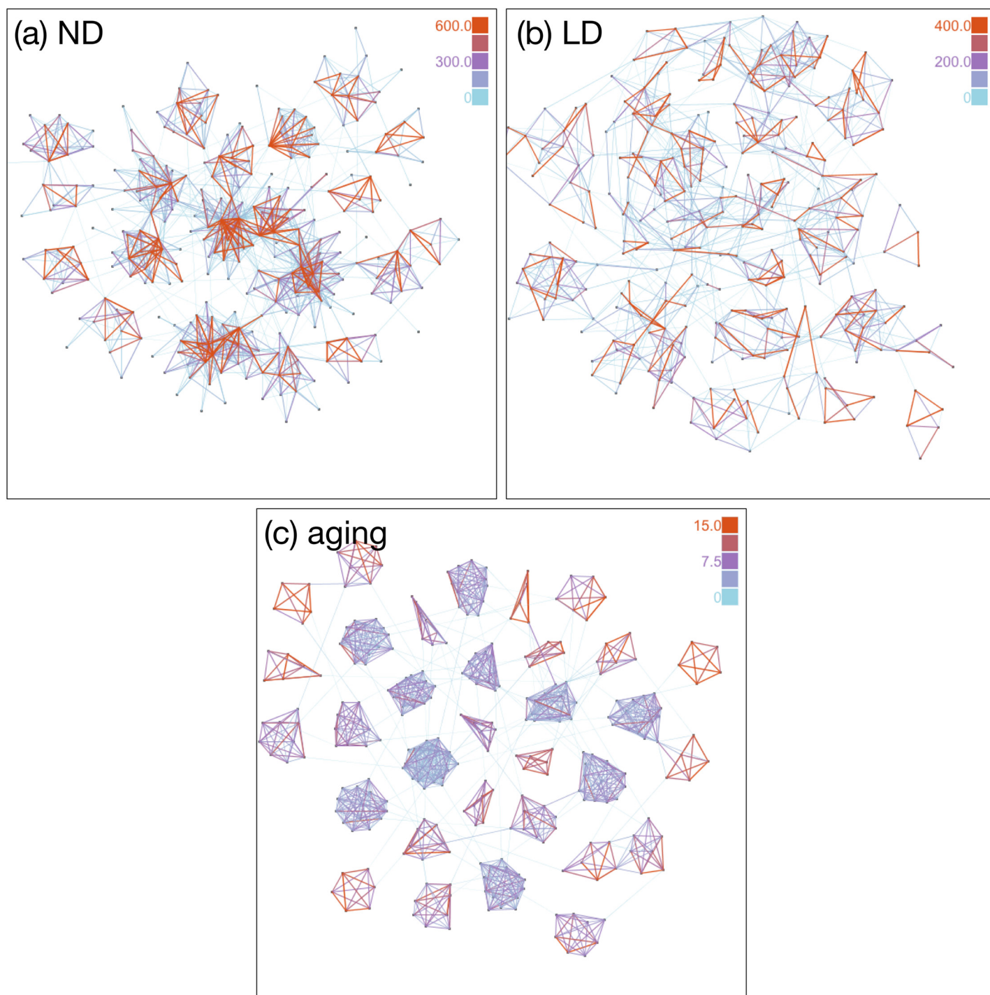
Fig 1. Network snapshots. Snapshots of typical network structures for (a) ND, (b) LD, and (c) aging mechanisms of link removals. Networks are drawn by using a force-directed graph drawing algorithm. Parameters are controlled such that these three networks have comparable average degrees (see Table 1). Color of links denotes the link weight. Strong and weak links are depicted in red and light blue, respectively. Note that different color scales are used for visibility. For the aging mechanism, community structures are clearly visible and the link weights in each community are more homogeneous. In the networks using the ND and LD mechanisms, strong and weak links coexist in each community.
