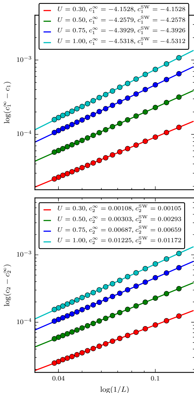
FIG. 2. The power-law dependence of c_1(L) (top plot) and c_2(L) (bottom plot) on 1/L plotted in log-log scale. The dots represent the DMRG results and the lines correspond to fitted function. Different colors correspond to different strengths of the attractive Hubbard interaction. Here, we set t = 1 . In the legends the values of c_{1(2)}^\infty and c_{1(2)}^{\text{SW}} are presented for a direct comparison.
