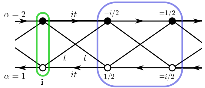
FIG. 1. The Creutz ladder: The green box indicates the i th unit cell containing two orbitals depicted by an empty and a full circle. The two sublattices are labeled by \alpha . The hopping amplitudes for the spin- \uparrow fermions are given on corresponding links. The arrows indicate the sense of the complex hoppings. The blue box indicates the maximally localized Wannier function for the upper/lower ( \pm ) flat band, also called plaquette states; the numbers correspond to the respective amplitudes which are nonzero only for the sites inside the blue box.
