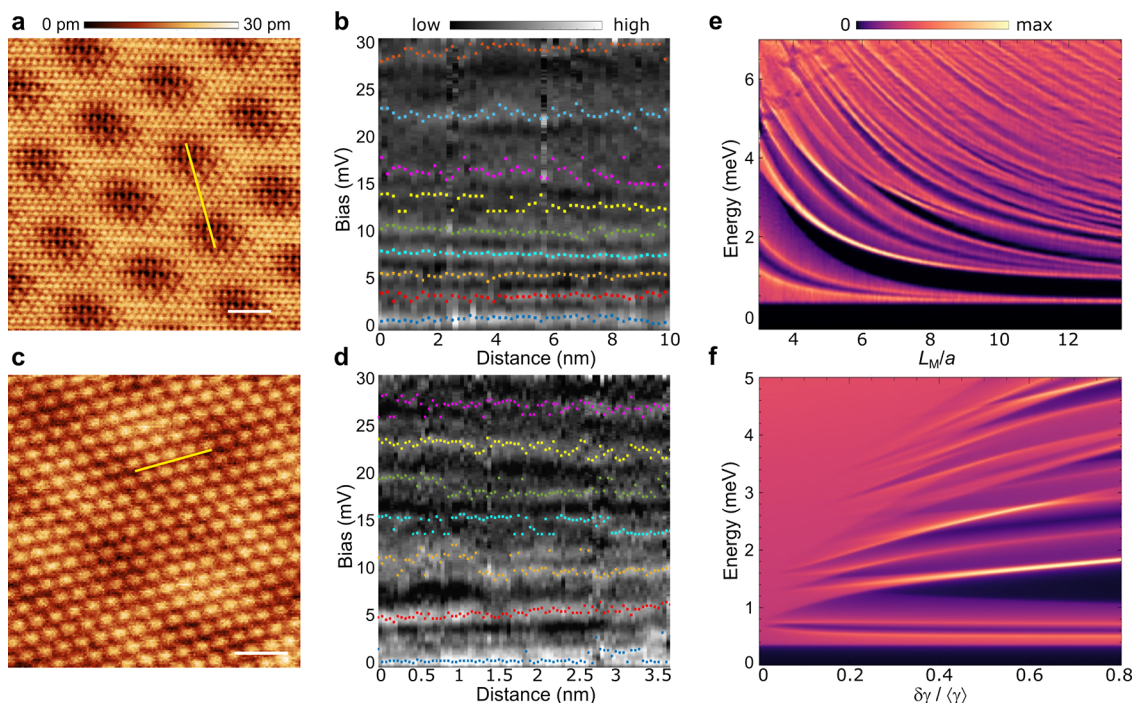
Figure 2. Moiré magnons in CrBr 3 . (a,b) Area with moiré wavelength 7 nm (Scale bar 4 nm. Image bias 1 V). Spatial dependence of antisymmetrized d^2I/dV^2 (b) with spectra taken along yellow line in panel (a). (c,d) Area with moiré wavelength 3.6 nm (Scale bar 2 nm. Image bias 2 V). Spatial dependence of antisymmetrized d^2I/dV^2 (d) with spectra taken along yellow line in panel (c). In (b),(d), colored points indicate the locations of maxima in the d^2I/dV^2 corresponding to the van Hove singularities in the magnon spectral function (see SI). (e,f) Theoretical dependence of the magnon spectral function with the moiré length (e) and with the strength of the exchange modulation (f).
