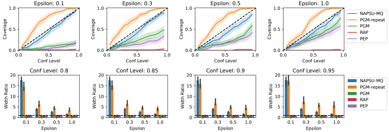
Figure 4: Top row: the fraction of downstream coefficients where the synthetic confidence interval contains the real data coefficient, averaged over 20 repeated runs on the Adult dataset using regularisation. NAPSU-MQ is the only algorithm that is consistently around the diagonal, showing good calibration. The error bands are bootstrap 95% confidence intervals of the average over the 20 repeats. Bottom row: confidence intervals widths divided by real data confidence interval widths. Each bar is a median over the different coefficients and repeats, and the black lines are 95% bootstrapped confidence intervals. The dashed line is at y = 1 , showing where synthetic confidence intervals have the same width as original confidence intervals. \delta \approx 4.7 \cdot 10^{-10} in all panels.
