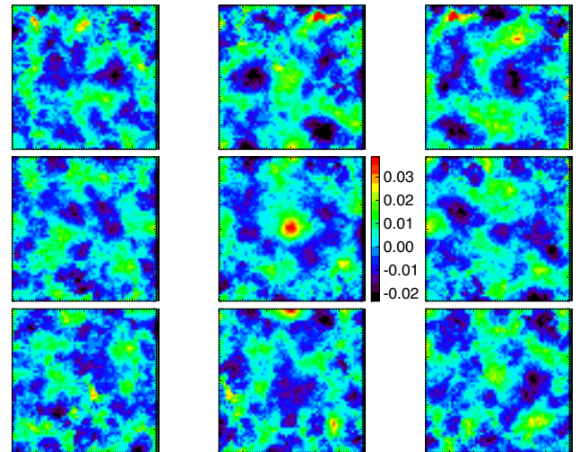
Fig. 3. Tests of stacking on “depainted” regions. The central panel shows the stacked result obtained at 857 GHz for the 645 cluster-centred patches (as in Fig. 2). This is surrounded by the eight neighboring maps obtained by changing the cluster Galactic longitude or latitude (or both) by \pm 1^\circ .
