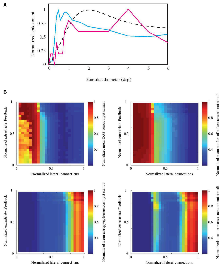
FIGURE 6 | Simulation result compared to natural ASF. (A) Examples of the spiking network response associated with high (solid blue curve) and low (solid red curve) efficiency measures to an increasing stimulus patch size, for a representative model neuron located at 14^\circ eccentricity. Response is averaged across 15 neighboring cells. The high-efficiency response is similar to ASF target at the same eccentricity (dashed curve) but with smaller summation field size. (B) Normalized mean distance to ASF (DAS), number of spikes, entropy per spike, and sparseness across all 20 natural images as a function of the number of V1 lateral excitatory-inhibitory and V1-extrastriate feedforward-feedback connections.
