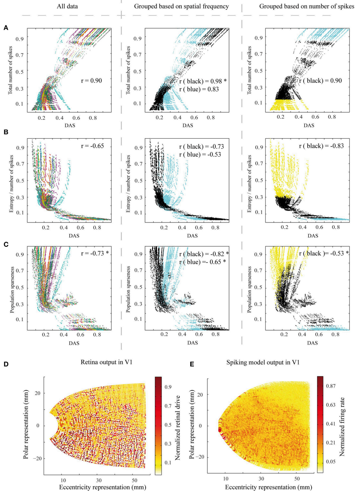
FIGURE 8 | The efficiency measures for a set of control simulations with a lower resolution of the retina filter. (A–C) The three efficiency measures as a function of DAS, as in Figures 7A–C . The color coding in the columns is the same as in Figures 7A–C . The correlation values differing significantly (Wilcoxon rank sum test with p < 0.05 ) from the original ones at Figure 7 are marked with *. (D) The low resolution retina function output for the Figure 2 , comparable to Figure 4F . (E) A sample of the corresponding simulated output pattern, comparable to Figure 4D . However, note that the color scale is different.
