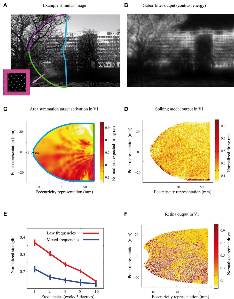
FIGURE 4 | The stimuli, predicted and simulated neural activation patterns. (A) The selected area of an example natural image illustrates the projection of the image to the Gabor filter and ASF calculations of the left visual field. Small dots in the pink square show the cortical density of cells in the visual field. The density of cells in each eccentricity follows the human cortical magnification factor. (B) The contrast energy image from the same natural image as in (A) , built as the output of a series of Gabor filters. These contrast images are the input for estimating the target area summation patterns. (C) The area summation target activation pattern, corresponding to the same natural image as in (A) . The color code of the activation pattern borders illustrates the projection of the image from the visual field to the model cortex, with the color code as in (A) . (D) Simulated output pattern for the image in (A) . (E) The normalized strength as a function of the spatial frequency contents for the natural images in Low and Mixed frequencies groups. Error bars represent the standard error of mean. (F) The output of the retina filter to the natural image in (A) , which served as an input to the spiking neural network simulations.
