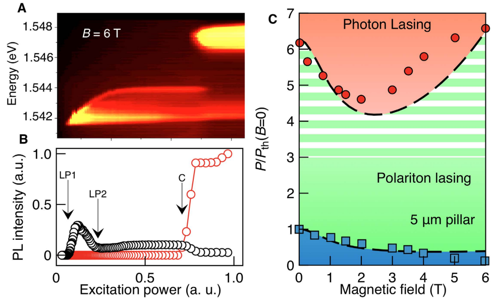
Figure 2. Phase transitions in micropillar samples. (a,b) Emission pattern and the integrated PL intensity of the 5 \mu\text{m} round pillar at B = 6\text{ T} . In (b) spectral integration has been performed over the polariton lasing peak (black circles) and photon laser peak (red circles), for details see Supplementary material. The arrows indicate the onset and offset of the polariton laser (LP1 and LP2) and the photon laser threshold (C). (c) Phase diagram of a 5 \mu\text{m} round pillar. The red circles correspond to the photon lasing threshold (C), the blue squares show the onset of polariton lasing (LP1). The offset of polariton lasing (L2) is shown only indicatively by the boundary between green color and white-green stripes. We cannot extract this threshold from the data with a high accuracy. Note that the polariton lasing transition for zero field reported in Fig. 2c corresponds to a pump power intermediate between those considered in Fig. 1a,b. The lines show the results of simulation. White horizontal bands mark the polariton gas regime, beyond the offset of polariton lasing.
