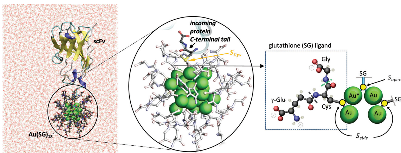
Fig. 2 Left panel: structure of the scFv...Au 25 (SG) 18 - complex (reactants state) obtained from MD and QM/MM simulations. Middle panel: zoom around the AuMPC. Color codes: Au (green), S (yellow), C (black), H (grey). The SG ligands are shown colorless. Right panel: schematic picture of one of the SG ligands bound in a dimeric staple of the gold cluster and atom labeling used in the manuscript text. The grey dashed line shows the gamma peptide linkage between glutamate and cysteine. The green dashed line shows the standard peptide linkage between cysteine and glycine.
