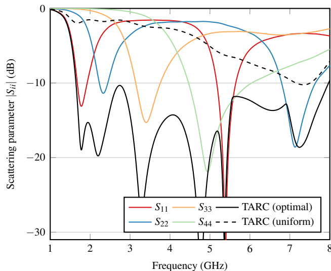
Fig. 3. Obtained TARC with optimized weights. TARC < -10 dB corresponds to a matching efficiency >90\% . The initial scattering parameters |S_{ii}| are shown for comparison.
