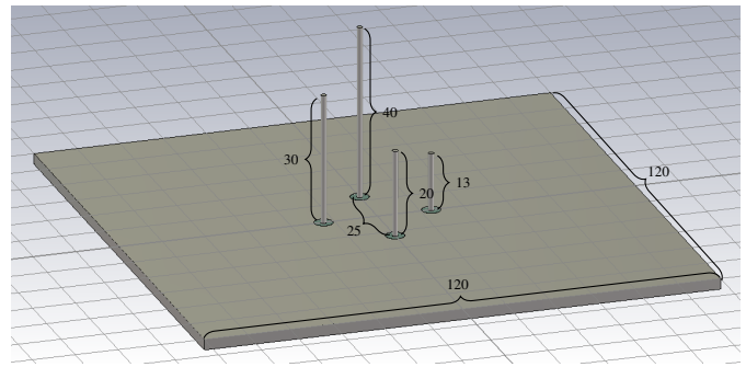
Fig. 2. Simulated antenna model in CST Microwave Studio. The monopoles are fed via coaxial connectors through the ground plane. All dimensions are in millimeters.
