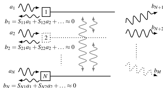
Fig. 1. The antenna concept presented in this letter. The antenna consists of multiple elements that have strong mutual coupling between them. By properly weighting the incident signals a_i in each element, the total reflected power can be minimized and matching efficiency maximized.
