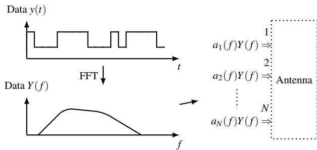
Fig. 5. Obtaining wideband operation. The frequency spectrum of the digital signal is split into several bands and the weights are calculated for each band and antenna element. The weighted signal is then fed to the antenna ports to obtain the wideband operation.
