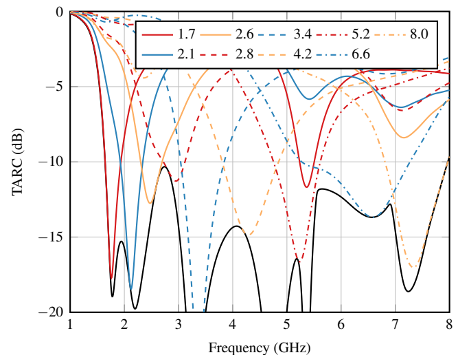
Fig. 4. An example for covering the frequency band from 1.65 to 7.95 GHz, with the criterion TARC < -10 dB. Each curve corresponds to an optimization point (frequency in GHz). The minimum obtainable TARC from Fig. 3, is also shown for reference. The minimum TARC is reached at the optimization points.
