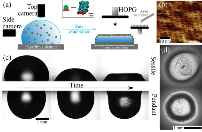
FIG. 1. (a) Sketch of the experimental setup. A droplet is placed on a Parafilm substrate and its shape is recorded from above and the side by cameras. After the formation of the flattened region, a highly ordered pyrolytic graphite (HOPG) substrate was brought in contact with the top of the droplet to perform imaging through an atomic force microscope (AFM). (b) AFM image of HFBI monolayer at the air-water surface. (c) Sessile (top) and pendant (bottom) droplet shapes at different times during evaporation. The initial volume is V_i = 13.1 \text{ mm}^3 in both cases, while the initial concentration of HFBI 2 \mu\text{mol L}^{-1} for the sessile drop and 4 \mu\text{mol L}^{-1} for the pendant drop. (d) Plan views of a crumpled sessile (top) and a wrinkled pendant (bottom) droplet.
