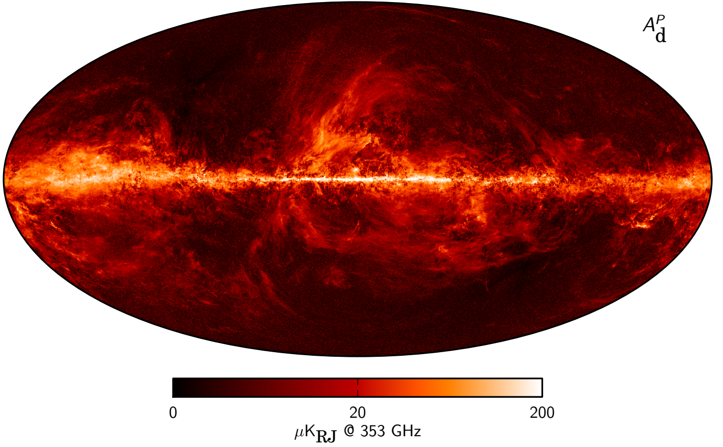
Fig. 24. Dust polarization amplitude map, P = \sqrt{Q^2 + U^2} , at 353 GHz, smoothed to an angular resolution of 10' , produced by the diffuse component-separation process described in Planck Collaboration X (2016) using Planck and WMAP data.
