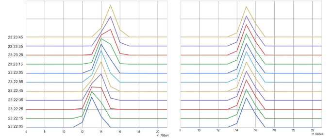
Fig. 10. Zoom into the carrier line without ( left panel ) and with the Doppler phase correction ( right panel ). 10 s integration time, 2^{15} = 32\,768 points spectral resolution, baseline Hh-Ww, scan 135. 23:22–23:24 UTC, December 28, 2013.
