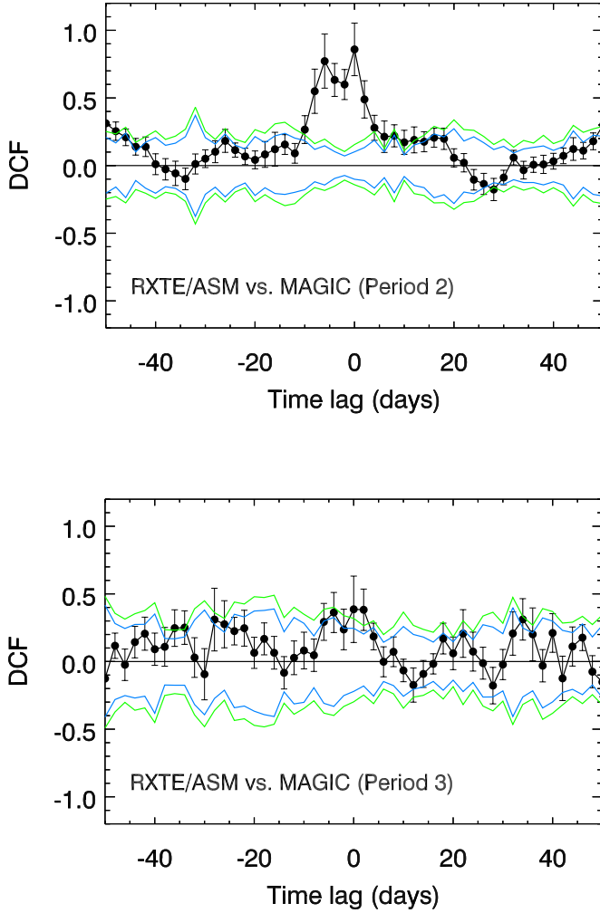
Fig. 6. Discrete correlation function for the light curves of RXTE/ASM and MAGIC for Period 2 (top) and for Period 3 (bottom). The description of data points and contours are given in the caption of Fig. 5.
