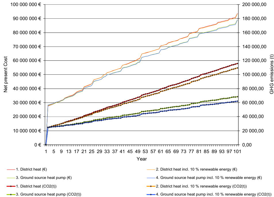
Fig. 1. Cumulative LCC and LCA outcome (100 years).
