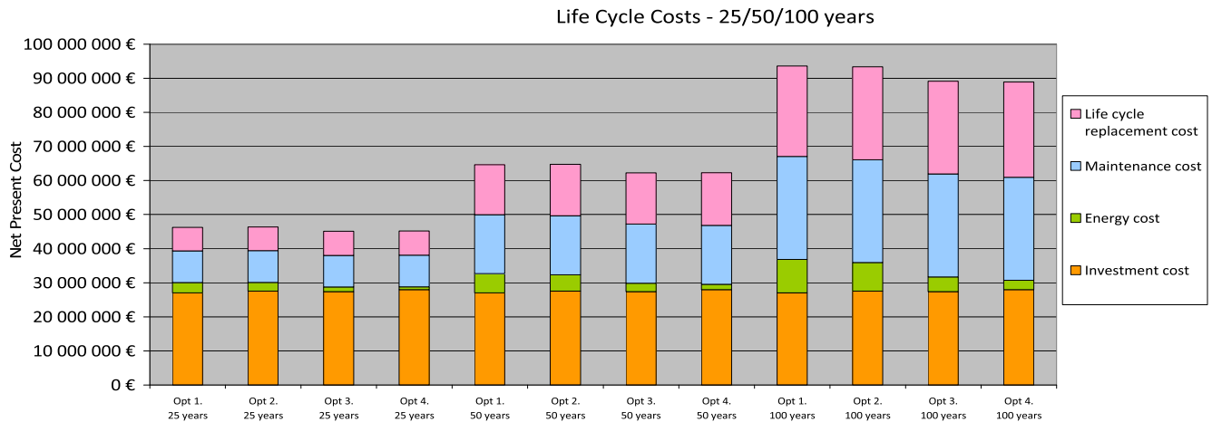
Fig. 2. Life cycle costs (NPC) for the evaluated options (25/50/100 years).
