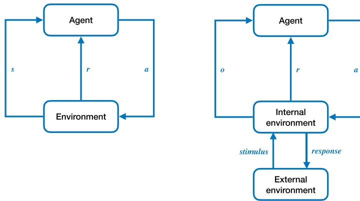
FIGURE 2 Illustrations of two alternative Markovian definitions of the computationally rational problems faced by humans. Left: An agent operating directly in the external environment. Right: an agent operating via its internal environment (Singh, Lewis, and Barto 2009) and yoked to the external environment by stimulus and response. When the latter is used to model humans, cognitive bounds are modeled as functions bounding observations ( o ), reward ( r ), and internal action ( a ). Here, the agent operates in an internal environment; it observes percepts, motor system, memory, fatigue, pain, stress, and so forth. Stimuli are perceived and represented in the internal environment and responses are caused by changes in the internal environment. The reward is a subjective utility function capturing the agents preferences.
