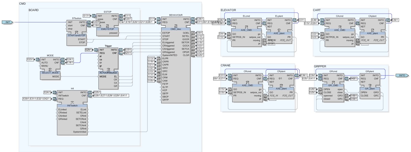
FIGURE 5. IEC 61499 global composite FB of the HHM model.
