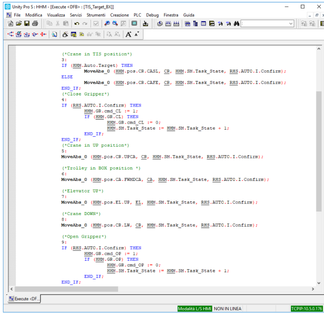
FIGURE 4. Original HHM control program, based on IEC 61131-3 structured text.
