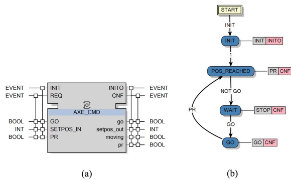
FIGURE 6. Overview of the controllers dedicated to the HHM linear motion axes and gripper. (a) AXE_CMD FB. (b) AXE_CMD ECC.
