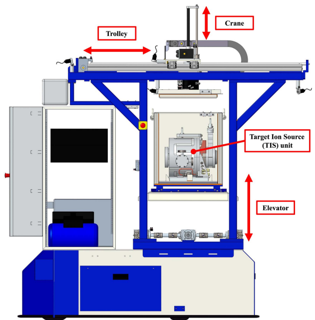
FIGURE 8. Graphical representation of the HHM CAT used in the HMI for online monitoring and simulations.
