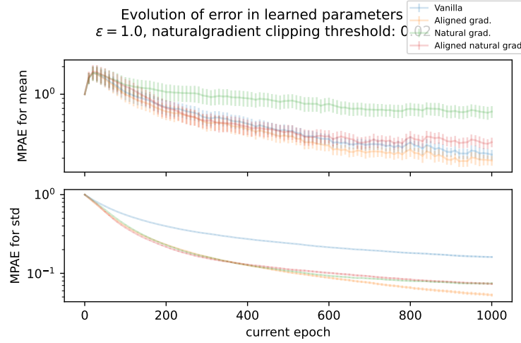
Figure H.3: The natural gradient based variants achieve comparable performance in terms of variational parameters for std but perform worse for variational means. This is strongly observable for the plain natural gradients while aligned natural gradients improve error in variational means in comparison. However, both are outperformed by (non-natural) aligned gradients in this experiment. Lines show the mean MPAE over 10 independent repeats as well as std. of mean as error bars. Clipping threshold for both natural gradient based variants is set to C = 0.02 , \sigma_q was initialised to 1. The natural gradient variant appears to diverge from the true variational std. which might be caused by clipping-induced bias, while still struggling to learn the correct variational mean.
