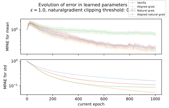
(b) Both natural gradient variants start to diverge if clipping is set too low C = 0.01 .
