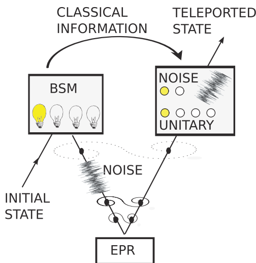
Figure 1 | A schematic picture of the teleportation protocol with nonlocal memory effects. EPR refers to a source producing states of the form of equation (1) and BSM refers to a Bell-state measurement. The local noise before the BSM makes the EPR pair mixed while the noise in the last step of the protocol allows to recover the teleported state.
