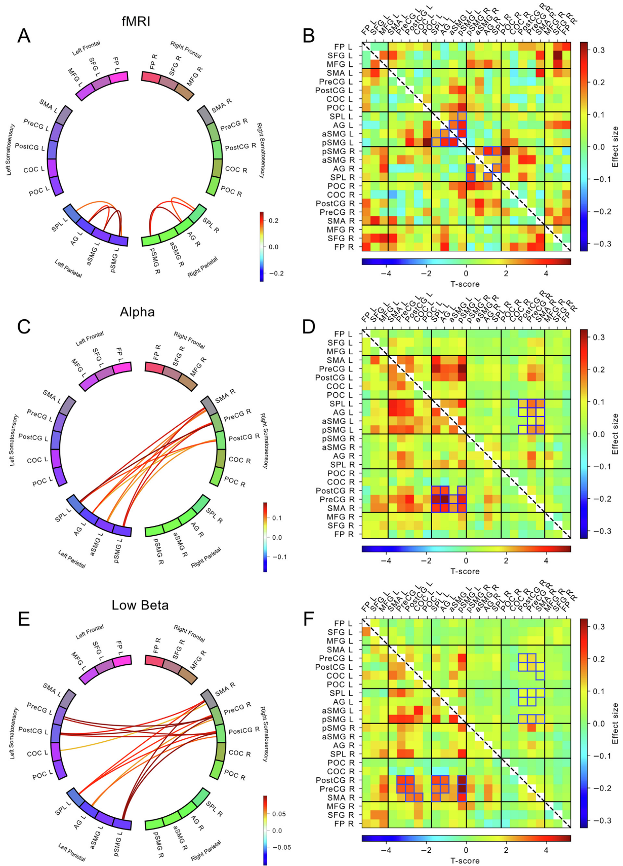
Fig. 2. Group differences (CP > control) in functional cortical connectivity for fMRI and MEG. Left: Connectivity circle with the post-hoc significant connections for (A) fMRI, (C) MEG alpha and (E) lower beta bands. Right: Group difference matrices for (B) fMRI, (D) MEG alpha and (F) lower beta bands with upper and lower halves showing the effect size and the post-hoc T-statistic respectively. The post-hoc significant differences ( p < 0.05 ) have been highlighted in blue. Refer to Table 3 for explanation of abbreviations.
