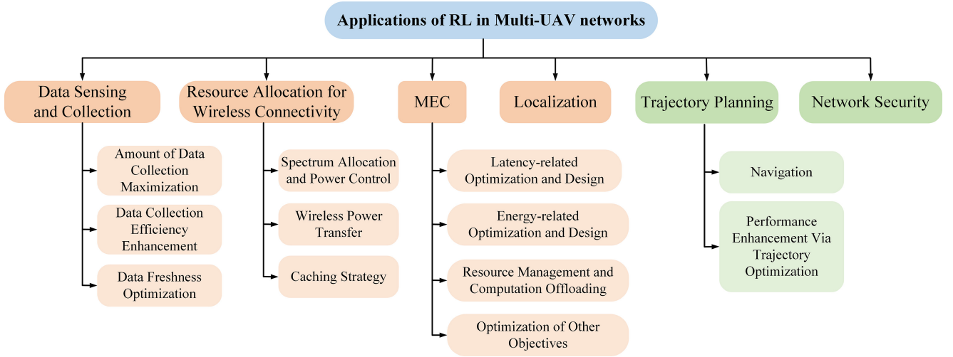
Fig. 2. A classification of the applications of RL in MUWNS.
