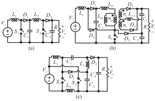
Fig. 9. Examples of multistage (cascaded) NHSDCs. (a) Two-stage cascaded boost converter. (b) Integrated structure [68]. (c) Integrated structure with more than one switch [189].
