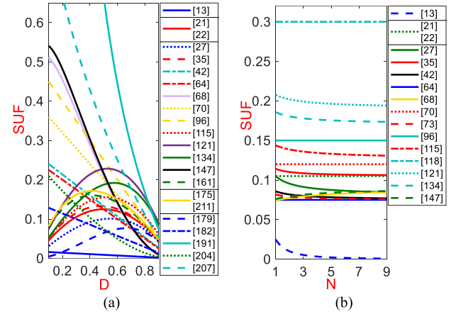
Fig. 23. SUF comparison of NHSDCs with regard to (a) D and (b) N .
