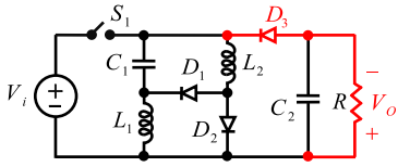
Fig. 15. Example of the inverted output voltage [200].
