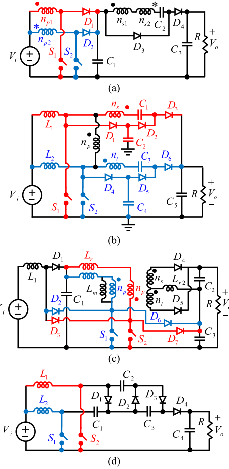
Fig. 10. Examples of interleaved NHSDCs with (a) common VMC [20], (b) separated VMCs [25], (c) interleaving in the input port of the second stage in a two-stage cascaded converter [105], and (d) integrated VMC [151].
