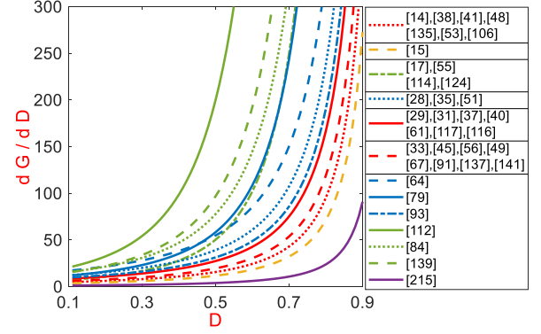
Fig. 28. Sensitivity comparison of voltage gain according to D variation.
