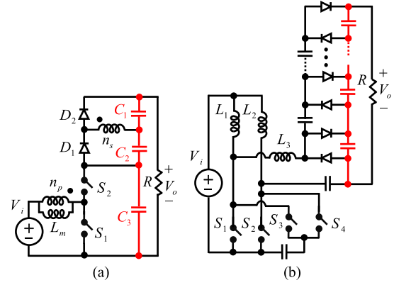
Fig. 11. Examples of multilevel NHSDCs. (a) Stacked structure [12]. (b) Extendable structure [150].
