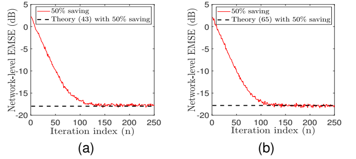
Fig. 7. Learning curves of the proposed PPD strategies: (a). Noise-injection-based PPD. (b). Decomposition- and noise-injection-based PPD.
