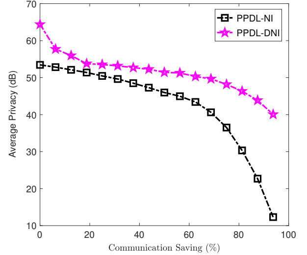
Fig. 6. Communication saving vs. average privacy for \sigma_v^2 = 4 .
