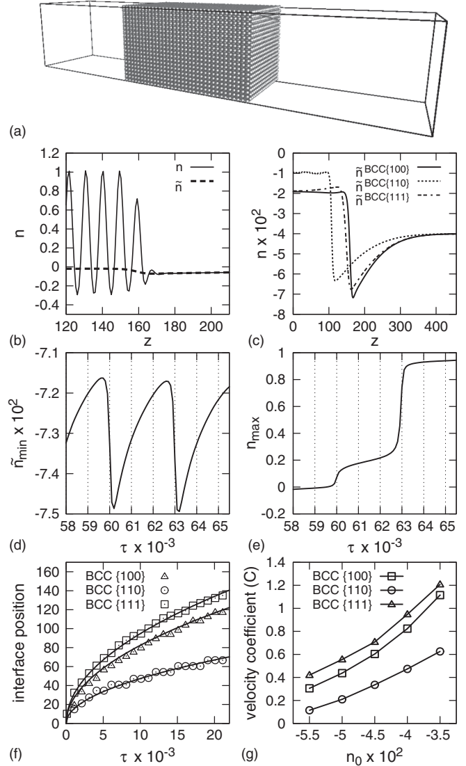
FIG. 2. bcc crystal growth as predicted by the PFC model. (a) Simulation box with crystal growing into the (100) direction. (b) Local and coarse-grained (filtered) densities across the \{100\} interface. (c) Coarse-grained densities for the \{100\} , \{110\} , and \{111\} interfaces. (d) Depth of the depletion zone vs dimensionless time ( \tau ) in (b). (e) Peak amplitude vs \tau for (b). (f) Interface position vs \tau and (g) the velocity coefficients vs n_0 for the three low index orientations.
