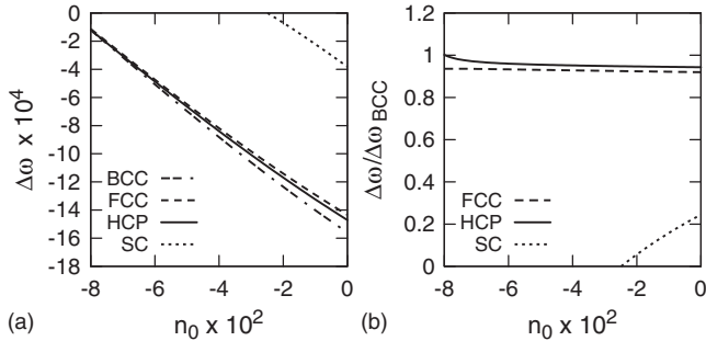
FIG. 1. (a) Driving force of crystallization, \Delta\omega , and (b) \Delta\omega/\Delta\omega_{bcc} vs initial number density for various polymorphs.
