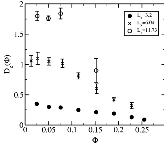
FIG. 11. The tracer diffusion coefficient in the z direction parallel to gravity.
