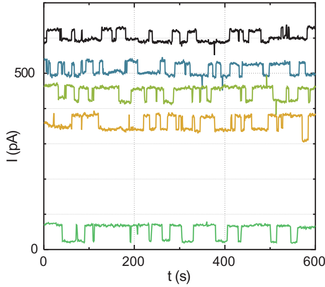
Figure 4. Random state switchings in sample 1, detected by the electrometer, biased to five different operation points and thus related to different levels of the dissipated power P \equiv I \times V_{\text{EM}} , V_{\text{EM}} being the bias voltage of the detector. From the bottom to the top: P \approx 0.03, 0.32, 0.44, 0.53 and 0.66 pW. The corresponding lifetime expectations, \tau = 25, 17.1, 17.6, 15.4 and 19.3 s, indicate only a weak influence of the electrometer on the trapping circuit.
