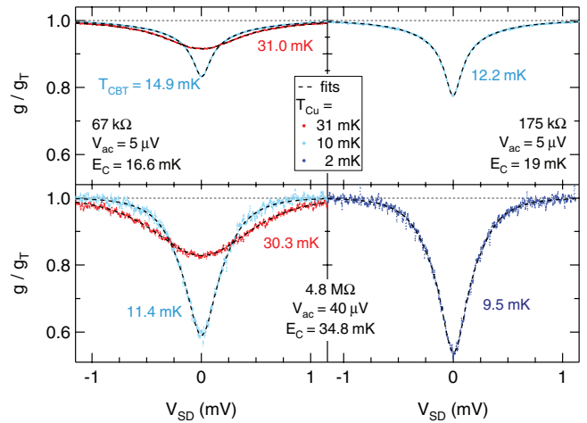
FIG. 2. CBT normalized differential conductance g/g_T versus source-drain dc bias V_{\text{SD}} for various NR temperatures T_{\text{Cu}} as color-coded, with resulting T_{\text{CBT}} ( \delta g method, see text) given adjacent to each trace. Data from a 67 k \Omega , 175 k \Omega , and 4.8 M \Omega CBT is shown. Dashed curves are fits to a model (see text). Note lower noise in low- R sensors due to larger resulting currents.
