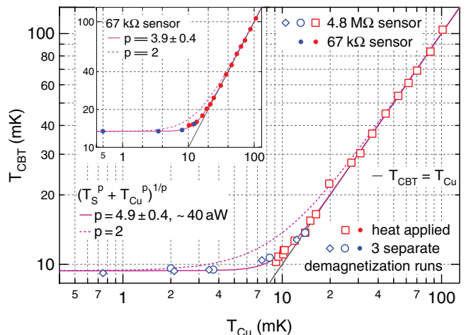
FIG. 3. CBT electron temperature T_{\text{CBT}} versus NR temperature T_{\text{Cu}} for 4.8 M \Omega (open markers) and 67 k \Omega sensors (filled markers, same axes on inset as main figure). Below 10 mK, the data are obtained in 3 demagnetization sweeps (blue markers) with B = 9 T, 5 T, 2 T, 1 T, and 0.4 T in a typical run, ramped at 1 T/h above 1 T and 0.5 T/h below. Error bars are about the size of the markers. Purple curves are T_{\text{CBT}} saturation curves (see text).
