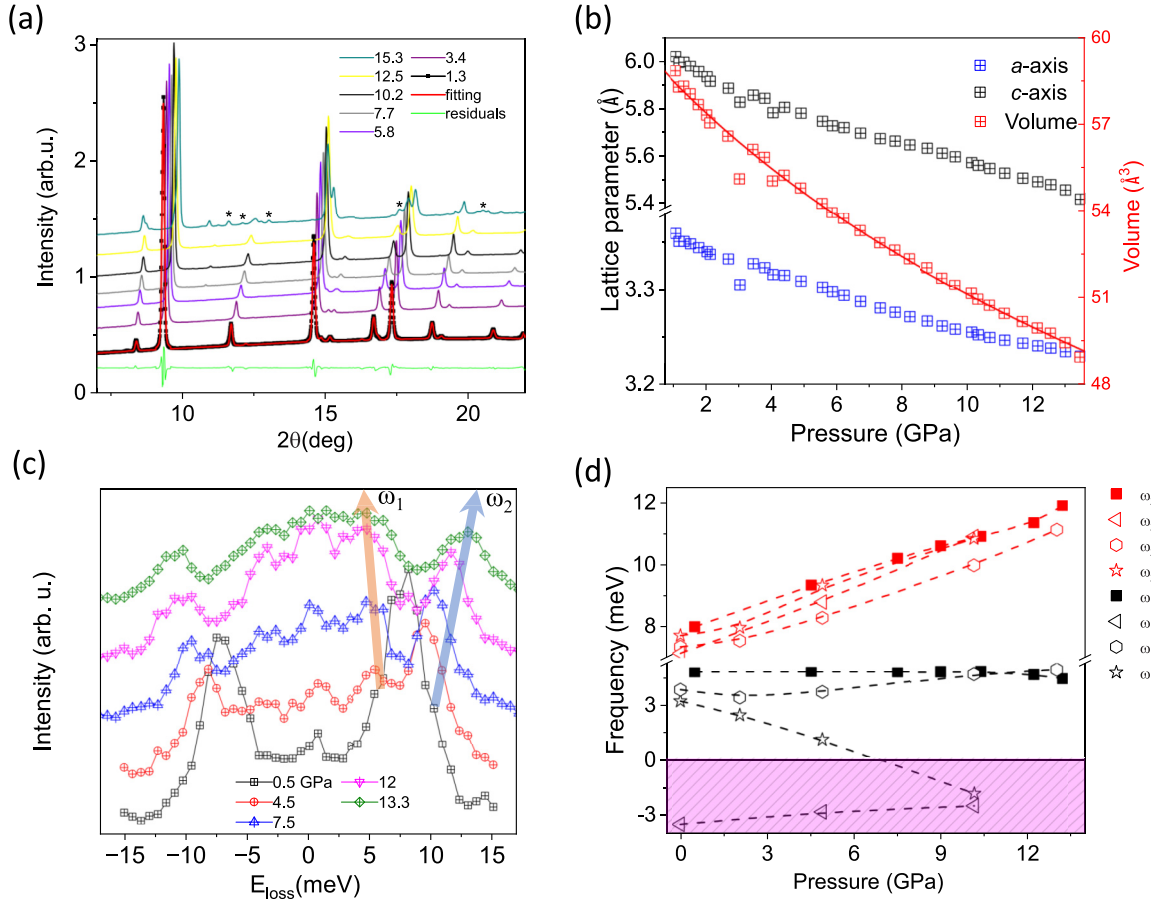
FIG. 14. (a) Representative x-ray diffraction scans as a function of pressure at 300 K. Peaks marked with an asterisk denote the new phase. The LeBail fitting to the experimental data is shown for 1.3 GPa. (b) Pressure dependence of the lattice parameters a and c . (c) Experimental pressure dependence of \omega_1 and \omega_2 at \mathbf{q}_{\text{CDW}} and (d) its comparison with SSCHA results from the free-energy Hessian including different vdW functionals.
