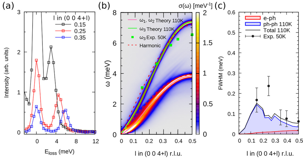
FIG. 10. (a) Representative momentum dependence of the IXS spectra at 50 K, (b) anharmonic spectral function compared to the experimental peaks and (c) linewidth of the longitudinal (0\ 0\ 4+l) r.l.u. phonon at 50 K in experiments and 110 K in anharmonic theoretical calculations.
