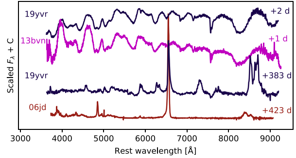
Figure 1. SN 2019yvr transitions from a SN Ib spectrum around maximum to a Type II-like spectrum at late phase. Comparison data include a similar phase spectrum of the SN Ib iPTF13bvn (Srivastav, Anupama & Sahu 2014) and the Type II SN 2006jd (Stritzinger et al. 2012). Spectra are corrected by redshift and not corrected by extinction.
