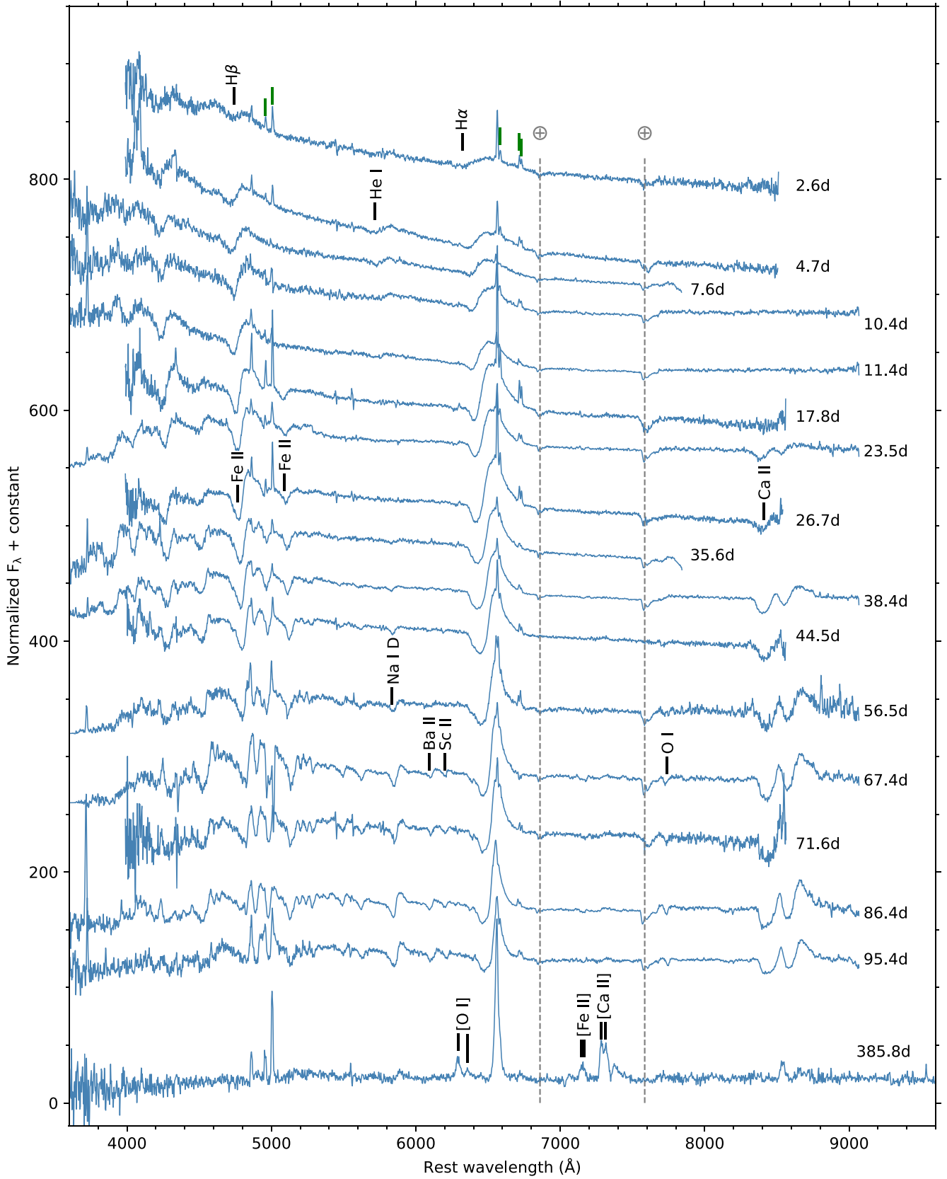
Figure 5. Spectral evolution of SN 2021gmj from 2.6 to 385.8 d after the explosion. The green lines represent [\text{O III}] \lambda\lambda 4959, 5007 , [\text{N II}] \lambda 6584 , and [\text{S II}] \lambda\lambda 6716, 6731 originating from the nearby H II region. The narrow Balmer lines are also due to the contamination from the nearby H II region.
