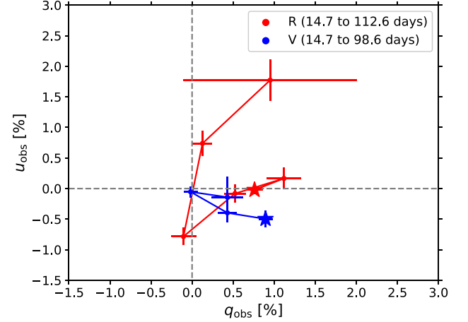
Figure 9. The observed Stokes parameters in the q-u plane. The first epoch in both bands is 14.7 d after the explosion. The final epoch in V and R bands is 98.6 and 112.6 d, respectively. The stars represent the values in the first epoch.
