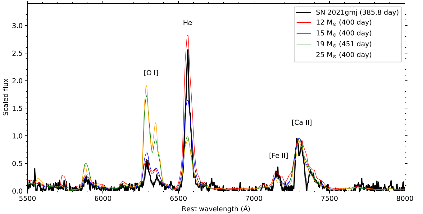
Figure 12. Comparison of the nebular spectrum of SN 2021gmj with the spectral models of Jerkstrand et al. (2014). Spectra are scaled to match the [Ca II] \lambda\lambda 7291, 7324 flux. The flux of narrow H \alpha from the host galaxy is subtracted from the observed flux assuming the flux ratio H \alpha /H \beta to be 3:1.
