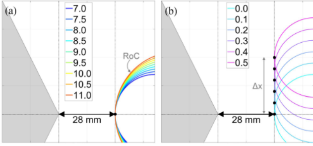
Fig. 3. Geometry for PO simulations of target RoC and transverse location. (a) Spherical target apex stays fixed at ~28 mm from the conical tip and the RoC is varied from 7.0 to 11.0 mm. (b) Target RoC is fixed and the apex is displaced transversely from the beam axis in steps of 0.1 to 0.5 mm. Coupling coefficients are computed for each of the perturbations described in (a) and (b).
