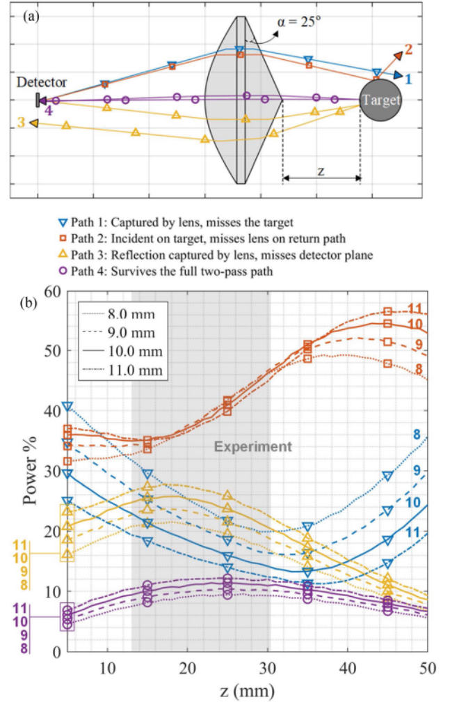
Fig. 2. (a) Nonsequential ray paths in the Zemax simulations. ( \nabla ) Captured by the lens but misses the target. ( \square ) Incident on target but misses lens on return path. ( \triangle ) Back reflection captured by lens but misses detector plane. ( \circ ) Survives the full two-pass path. (b) Nonsequential ray tracing power distribution on different path as a function of target distance. The simulation was repeated for sphere of different radii (paths of different colors) and at different positions of its apex. z is the distance between the axicon tip and the sphere apex.
