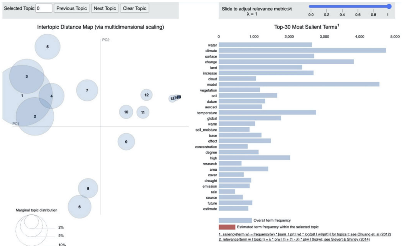
Figure 2. Visualization of topic distribution (left), and full list of keywords for the overall topic analysis (right). This visualization was created using the pyLDavis Python package. Note that visualizations for each individual topic are included in the Supplementary material.
