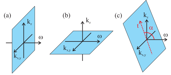
FIG. 3. (Color online) Slices of the 3 + 1-dimensional space (\omega, k_x, k_y, k_z) that are used to define the topological invariants for the (a) 3D {}^3\text{He-B} phase, (b) 2 + 1-dimensional planar phase, and (c) smooth transformation between 3D and 2 + 1-dimensional invariants. The auxiliary axis is t = \omega \cos \alpha + k_z \sin \alpha .
