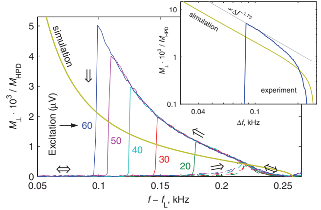
FIG. 3 (color). Formation of the magnon condensate in the ground state of the trap in Fig. 1 in cw NMR measurement. The condensate magnetization M_{\perp} precessing in the transverse plane is plotted on the vertical axis, normalized to that when the homogeneously precessing domain (HPD) fills the volume within the detector coil [23]. The arrows indicate the sweep direction of the applied rf frequency f = \omega/(2\pi) . M_{\perp} grows when the frequency is swept down. Only a tiny response is obtained on sweeping in the opposite direction. During the downward frequency sweep the condensate is destroyed (vertical lines), when energy dissipation exceeds the rf pumping. This point depends on the applied rf excitation amplitude, marked at each vertical line. The lower green line represents the result of calculations from Fig. 2. These calculations have no fitting parameters: the vertical difference from the measurements can be attributed to the experimental uncertainty in determining the normalization for M_{\perp} . Inset: The experimental curve measured with the largest excitation and compared to the numerical curve from the main panel, replotted with logarithmic axes to demonstrate the asymptotic limit for large magnon numbers: M_{\perp} \propto [f - f_L(0)]^{-1.75} , which corresponds to the condensate in a box.
