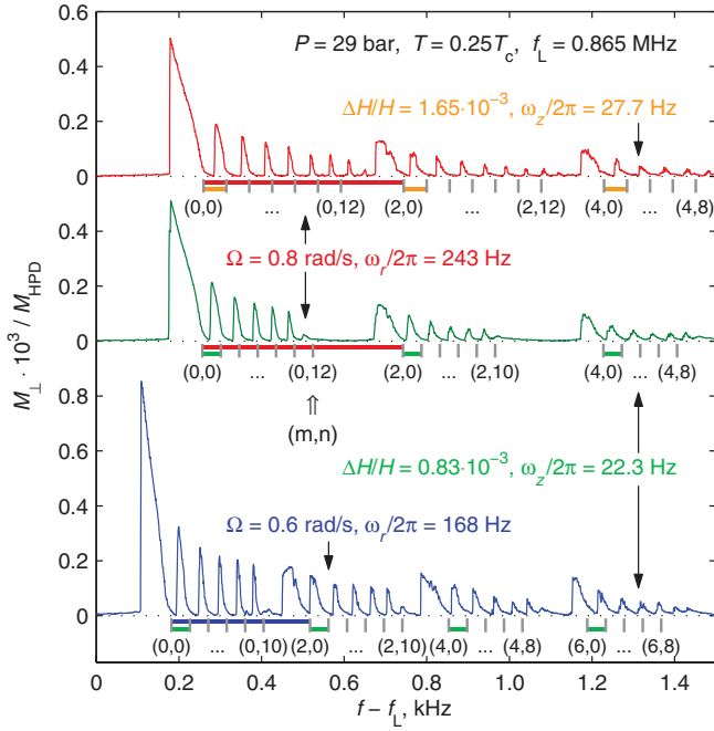
FIG. 4 (color). Formation of magnon condensates at different excited levels (m, n) of the magnetic trap in Fig. 1. When the frequency of the rf excitation field is swept down and crosses one of the levels (m, n) at f_{mn} , the magnon condensate starts to grow according to Eq. (7). Only modes with even m and n are excited. The three examples of measured spectra are for different values of rotation velocity \Omega in the vortex-free state and for different depths \Delta H/H of the axial field minimum in the trap. In the topmost case the depth of the field minimum is twice that of the two bottom examples. As a result, the smaller axial level spacing increases, as the axial oscillator frequency \omega_z/2\pi : 22 \rightarrow 27 Hz, but the larger radial level spacing remains unchanged. Similarly, when \Omega is increased from 0.6 rad/s (bottom spectrum) to 0.8 rad/s (two top most spectra), the radial level separation increases, as \omega_r/2\pi : 170 \rightarrow 240 Hz. The equidistant vertical tick marks refer to the level positions in the absence of magnons and have been fitted to the harmonic trap relation in Eq. (4).
