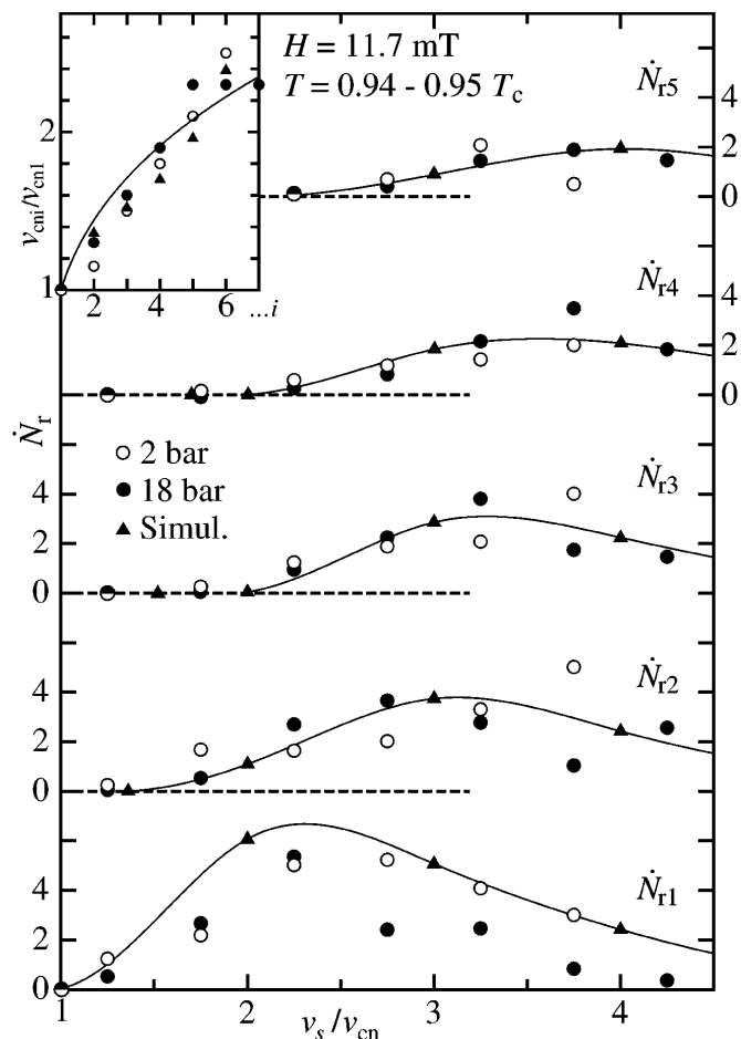
FIG. 3. Rates \dot{N}_{ri} of vortex line formation, grouped according to the number of lines i formed per absorption event per minute, plotted vs v_s/v_{cn} . The solid curves are spline fits to the simulation data. (Inset) Threshold velocity v_{cni}/v_{cn1} for the onset of an event with i lines, plotted vs the number of lines i . The solid curve represents the fit v_{cni}/v_{cn1} = [2.0(i - 1) + 1]^{1/3} .
