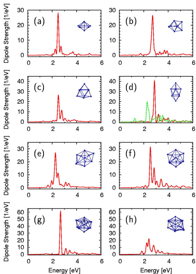
FIG. 2. (Color online) TDLDA spectra of the clusters \text{Na}_7 – \text{Na}_{14} . Note the different scalings of the axes of ordinates. For \text{Na}_{10} (d), spectra of a D_{4d} (red/solid) and a trigonal pyramidal (tetrahedral) isomer (green/dashed) are shown.
