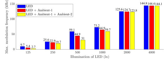
Fig. 4. Modulated light frequency response of the BD.
