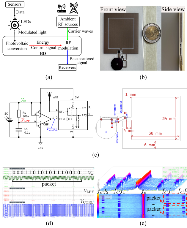
Fig. 1. BD. (a) Combination of VLC and AmBC. (b) Prototype after additive manufacturing. (c) Schematic and footprint layout. (d) Circuit outputs example. (e) Received signals in OTA demonstration.
