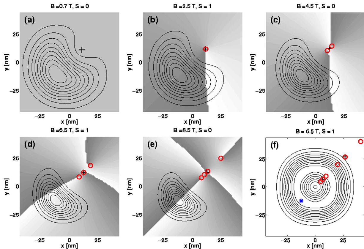
FIG. 18. (Color online) (a)–(e) Contours of conditional densities |\psi_c(x,y)|^2 and phase of the conditional wave function \theta_c(x,y) in grayscale for the L_x=5 , L_y=5 four-minima QDM. See Fig. 6 for details. (f) Contours of total electron density of the three-vortex triplet state are plotted in the background and positions of the vortices with the fixed electron in two different positions.
