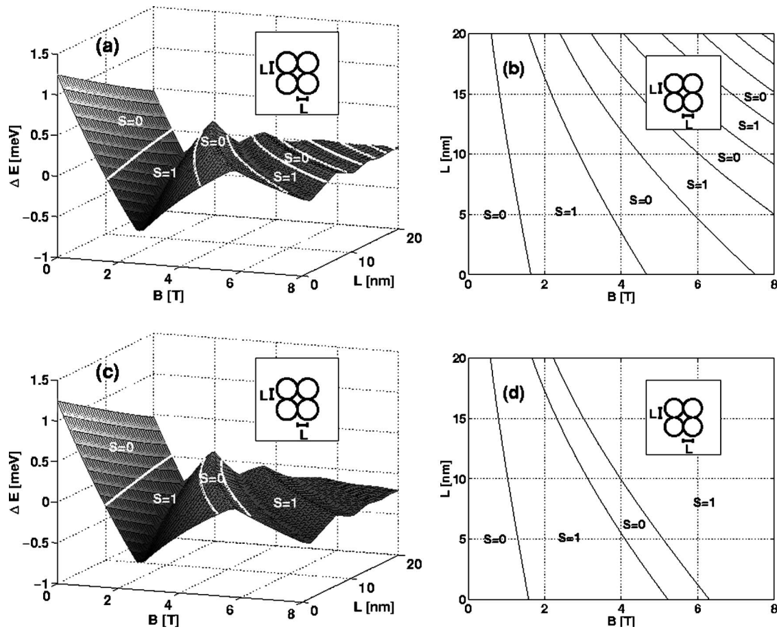
FIG. 15. Triplet-singlet energy difference ( \Delta E = E^{\uparrow\uparrow} - E^{\uparrow\downarrow} ) as a function of magnetic field in the square-symmetric ( L_x = L_y ) four-minima quantum dot molecule. See Fig. 9 for details.
