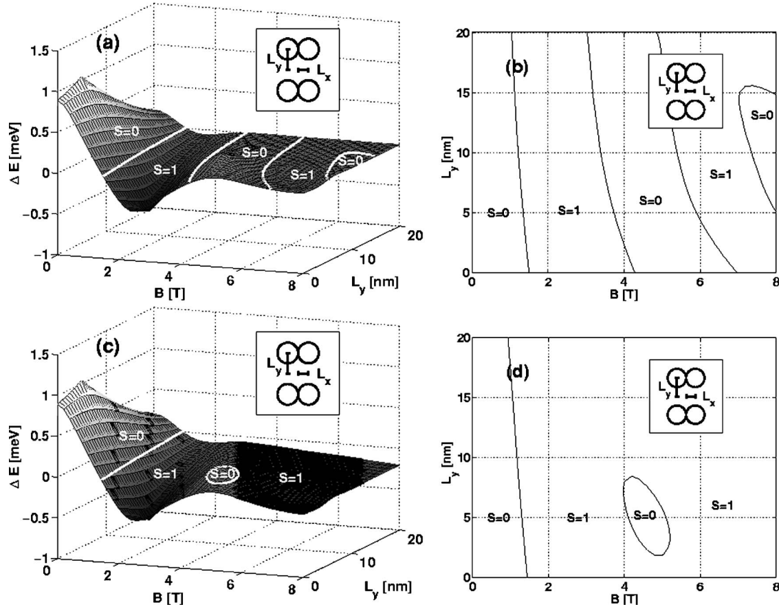
FIG. 21. Triplet-singlet energy difference ( \Delta E = E^{\uparrow\uparrow} - E^{\uparrow\downarrow} ) as a function of magnetic field in the rectangular-symmetric four-minima quantum dot molecule. L_x is fixed to 5 nm and L_y is varied from 0 to 20 nm. Therefore at L_y=0 we have L_x=5 nm double dot and at L_y=5 nm it is the square-symmetric four-minima QDM. The energy difference is plotted as a function of L_y and magnetic field in (a) without Zeeman energy and in (c) with the Zeeman energy included ( \Delta E = E^{\uparrow\uparrow} + E_Z - E^{\uparrow\downarrow} ). In (b) and (d) the ground state regions of the singlet and triplet states are plotted as a function of B and L_y , without and with Zeeman energy, respectively.
