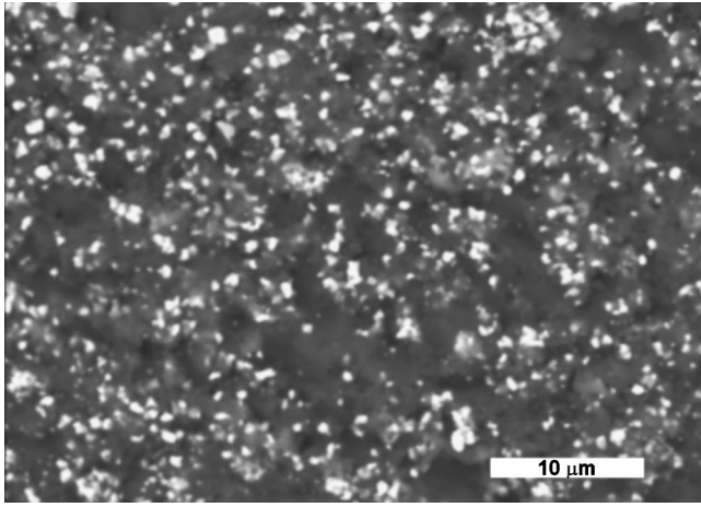
FIG. 3. Microstructural image of ceramic/epoxy composites with a ceramic loading of 10 vol %.
