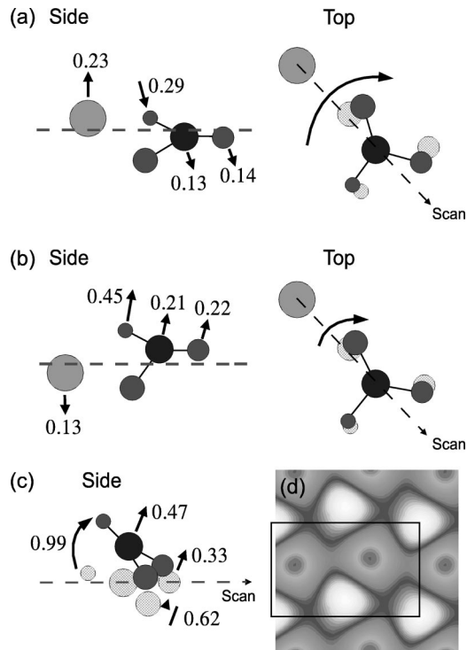
FIG. 22. Schematic diagrams of atomic displacements of the calcite ( 10\bar{1}4 ) surface as the tip scans across at 0.425 nm [(a) and (b)]. The numbers are in Å, and show the displacements when the tip is directly over that atom. Dark gray, C atoms; light gray, Ca atoms; and medium gray, O atoms. The size of the oxygen atoms in the carbonate group is in perspective, i.e., the larger the atom the further “out” of the page it lies. The cross-hatched atoms in some drawings show the undisplaced position of the atoms when the tip is not in proximity, and the arrows give an indication of the displacement direction as the tip approaches. (a) Scanning with a negative potential tip. (b) Scanning with a positive potential tip. (c) Scanning at 0.4 nm from the surface with a positive potential tip causes the whole carbonate group to flip up from the surface. (d) Density-functional theory (DFT) calculated electrostatic potential at 0.250 nm above the calcite surface in a plane parallel to C, Ca, and middle O atoms in the surface. The black rectangle is the unit cell of the ( 10\bar{1}4 ) calcite surface.
