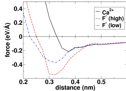
FIG. 20. (Color in online edition) Simulated force curves taken over the Ca, high and low F sites in the \text{CaF}_2 (111) surface with a pure silicon tip. Reprinted with permission (Foster et al. , 2002).
