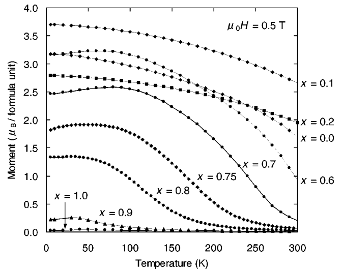
FIG. 2. Magnetic moment vs temperature for \text{Sr}_2\text{Fe}(\text{Mo}_{1-x}\text{W}_x)\text{O}_{6-w} .
