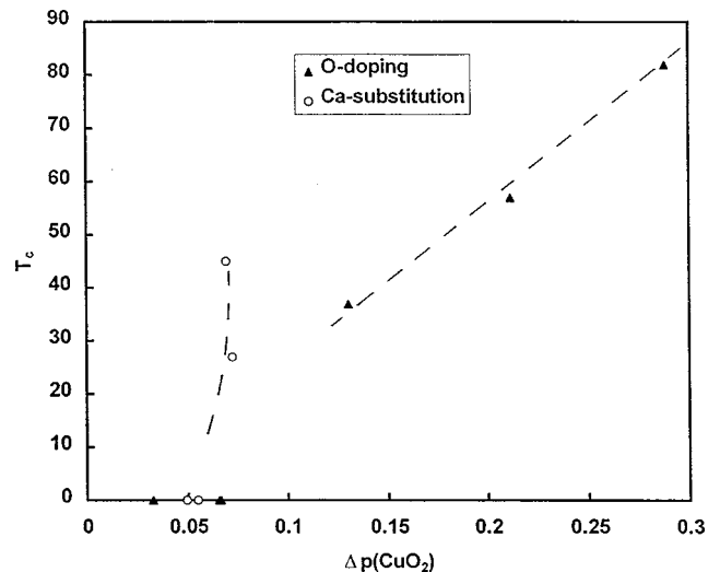
FIG. 5. T_c vs \Delta p(\text{CuO}_2) for the Ca-substituted ( z \approx 0 ; ○) and O-doped ( x = 0 ; ▲) \text{Cu}(\text{Ba}_{0.8}\text{Sr}_{0.2})_2(\text{Yb}_{1-x}\text{Ca}_x)\text{Cu}_2\text{O}_{6+z} samples.
