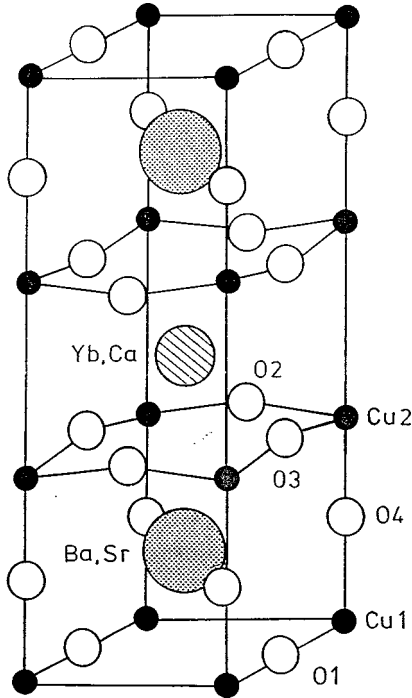
FIG. 2. Schematic presentation of the \text{Cu}(1)(\text{Ba}_{0.8}\text{Sr}_{0.2})_2(\text{Yb}_{1-x}\text{Ca}_x)\text{Cu}(2)_2\text{O}_{6+z} crystal structure and the present notation system for the atoms.
