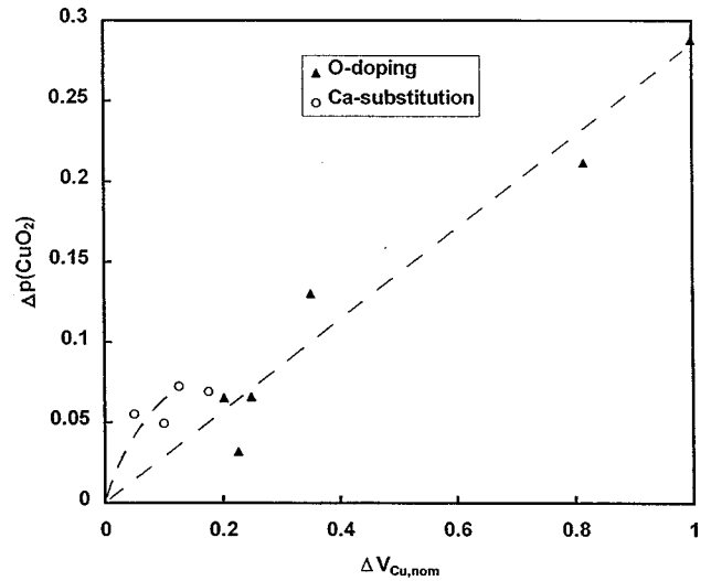
FIG. 4. \Delta p(\text{CuO}_2) vs \Delta V_{\text{Cu,nom}} for the Ca-substituted ( z \approx 0 ; ○) and O-doped ( x = 0 ; ▲) \text{Cu}(\text{Ba}_{0.8}\text{Sr}_{0.2})_2(\text{Yb}_{1-x}\text{Ca}_x)\text{Cu}_2\text{O}_{6+z} samples.
