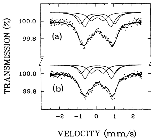
FIG. 7. Room-temperature Mössbauer spectra measured of samples with the nominal nonstoichiometric composition of 4:3:3:4 after the heat treatments of (a) 877^\circ\text{C} (10 h) and (b) 884^\circ\text{C} (100 h).
