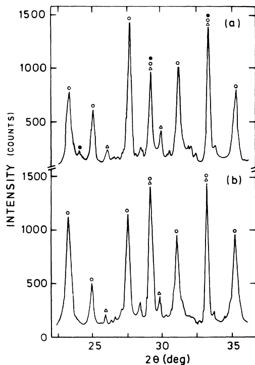
FIG. 3. \text{Cu-K}\alpha x-ray-diffraction data of (a) nondoped and (b) iron-doped ( x=0.01 ) samples with the composition 2:2:2:3 (final sintering at 877 °C for 10 h). The symbols \Delta , \circ , and \bullet denote the peaks corresponding to phases with T_c 's of 10, 80, and 110 K, respectively.
