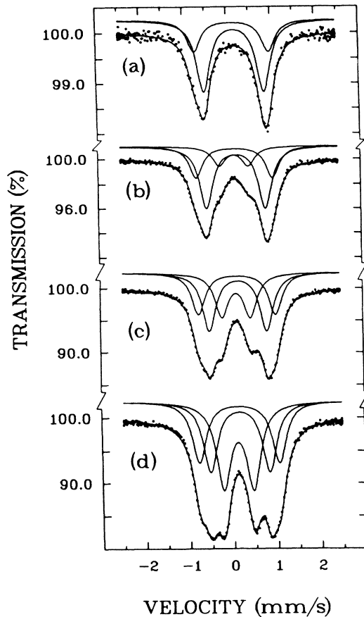
FIG. 6. Influence of iron doping on the Mössbauer spectra of samples with composition n=3 after the heat treatment of 884^\circ\text{C} . Spectra were measured at room temperature using various iron concentrations of (a) 1, (b) 5, (c) 10, and (d) 20 at. %.
