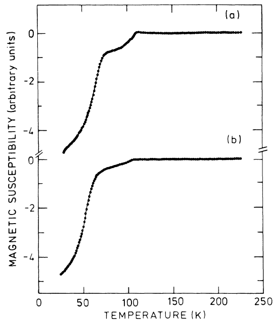
FIG. 2. Influence of iron doping on the compound corresponding to nominal composition n=3 . The samples were sintered at 877 °C for 10 h. Compared to the nondoped sample (a) the amount of the 110-K phase in the 1 at. % doped sample (b) is significantly reduced.
