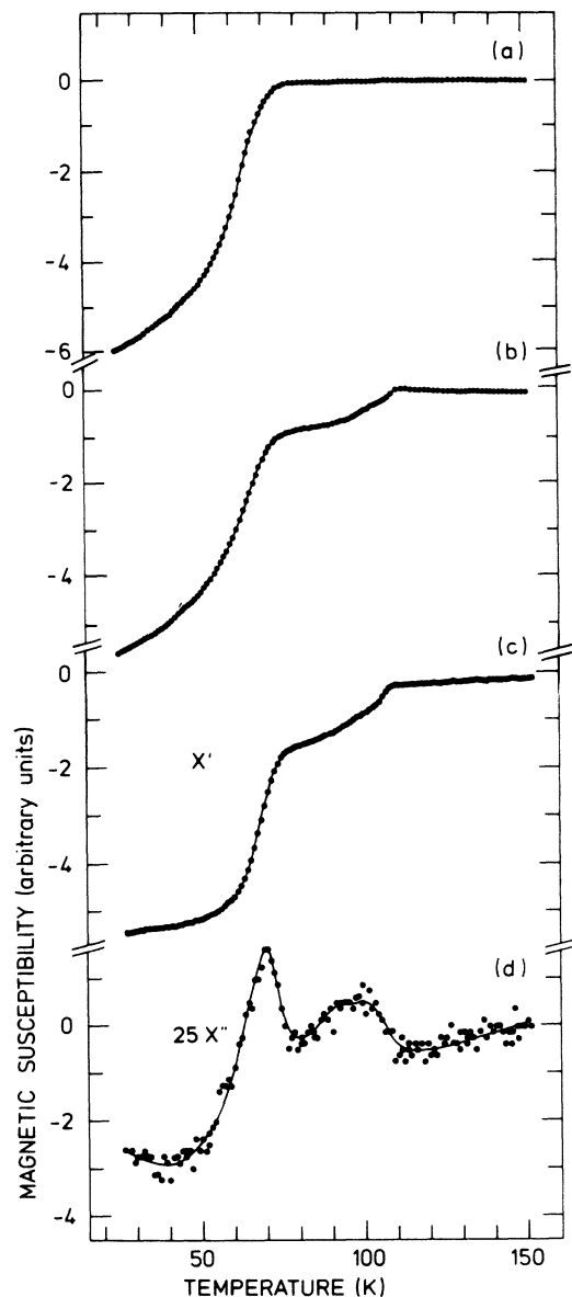
FIG. 1. Results of the magnetic ac susceptibility measurements of the influence of the nominal starting compositions on the superconducting properties of the \text{Bi}_2\text{Sr}_2\text{Ca}_{n-1}\text{Cu}_n\text{O}_{4+2n} compounds. a–c present the real part \chi' of susceptibility of samples corresponding to compositions (a) 2:2:1:2, (b) 2:2:2:3, and (c) 2:2:3:4. (d) shows the imaginary part \chi'' of the sample with the composition of 2:2:3:4. The final sintering temperature has been 877 °C (10 h).
