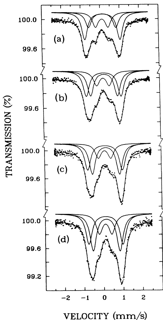
FIG. 4. Room-temperature Mössbauer spectra measured of samples with the nominal stoichiometric composition of n=2 after heat treatments of (a) 825^\circ\text{C} , (b) 877^\circ\text{C} , (c) 884^\circ\text{C} , and (d) 884^\circ\text{C} (100 h). The ^{57}\text{Fe} doping level was 1 at. %.
