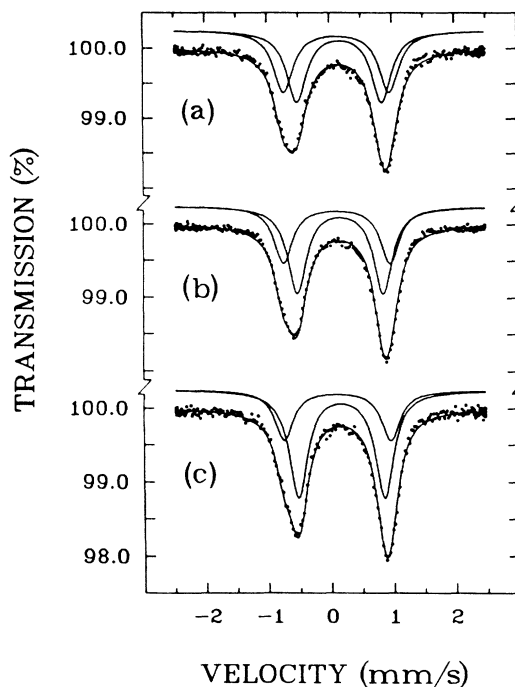
FIG. 5. Spectra measured of samples with nominal stoichiometric composition of n=3 after heat treatments of (a) 877^\circ\text{C} , (b) 884^\circ\text{C} , and (c) 884^\circ\text{C} (100 h).
