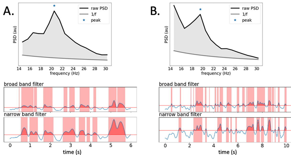
Fig. 4. Effect of broad-band (14–30 Hz) vs. narrow band (peak frequency \pm 2 Hz) filtering on amplitude envelope and signal to noise ratio (SNR), shown for a prominent (A) and a weaker (B) beta range spectral peak. The selection of the individual peak and bandwidth has relatively more effect in the prominent peak case in which the SNR decreases with increasing filtering bandwidth. Note that the y-axis is in non-logarithmic scale.
