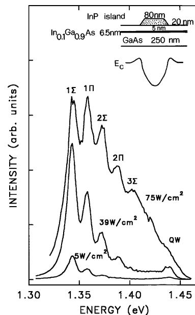
FIG. 1. Photoluminescence spectra of InGaAs quantum dots excited with an argon laser. For I_{\text{exc}} = 75 \text{ W/cm}^2 we estimate, on the basis of peak intensities, that there are approximately 6–8 electrons and 6–8 holes in a quantum dot. Inset: schematic diagram of the strain-induced confining potential of the dots.
