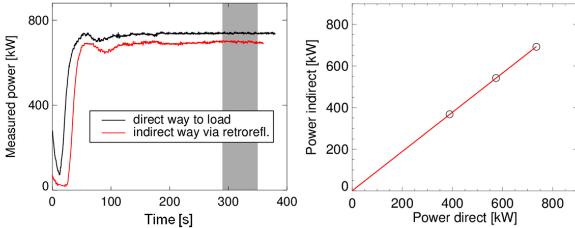
Figure 4. The left hand side shows the measurement of the gyrotron power, comparing the power level of the direct way to the load with the level of the indirect way via a retro-reflector. The inferred transmission efficiency is 94%. Repeating the measurements at different power levels results in a linear dependence (right hand side figure) allowing a robust determination of the power loss.
