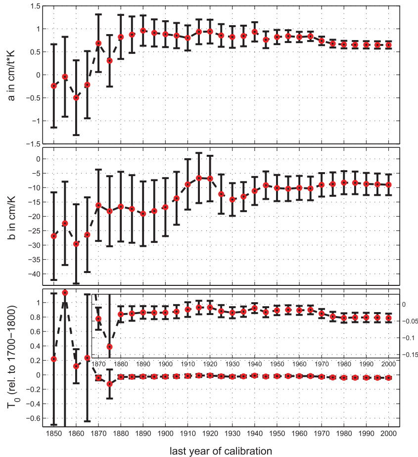
Figure 2. Parameter dependency on calibration period. The parameters a , b and T_0 from (1) with 1 \sigma error shown over the last year of calibration, on the JE08 data, starting 1700. The inset in the lower panel expands the vertical scale.
