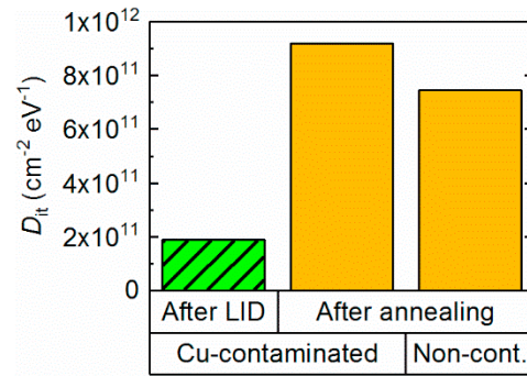
Fig. 5. Density of interface traps ( D_{it} ) in Cu-contaminated samples ( [\text{Cu}] = 5 \times 10^{13} \text{ cm}^{-3} ) both after LID and after annealing, and in a reference non-contaminated sample after annealing. The annealing step increases D_{it} approximately similarly both in the Cu-contaminated and the non-contaminated samples.
