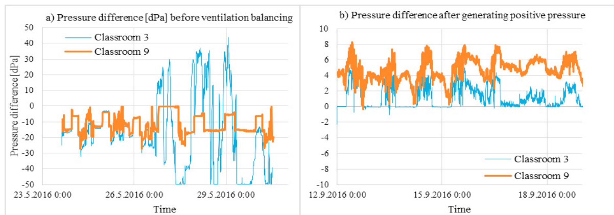
Fig. 3. Pressure differences (indoor-outdoor) in classrooms 3 and 9: (a) before ventilation system balancing and (b) after ventilation system balancing and generating positive pressure.
