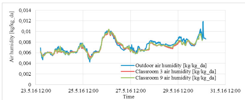
Fig. 4. Air humidity (kg per kg of dry air) in classrooms 3 and 9 and outdoors.
