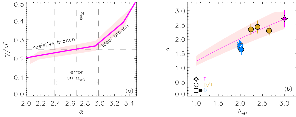
Figure 17. (a) Growth rate of the most unstable mode, relative to diamagnetic frequency \omega^* , versus maximum normalized pressure gradient \alpha , from resistive linear MHD stability. The calculation is for the experimental value of pedestal current density j of the T pulse of the D-T scan; (b) variation of \alpha vs A_{\text{eff}} : experiment (symbols) vs critical \alpha (solid line). Reproduced from [91]. © 2023 The Author(s). Published by IOP Publishing Ltd on behalf of the IAEA. All rights reserved. CC BY 4.0 .
